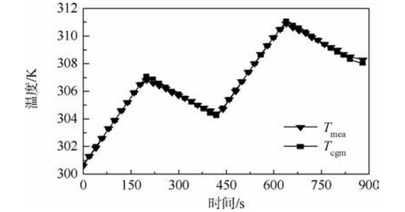
图 5 数值试验 2 的温度反演值与测量值比较 Fig. 5 Compare between inversion temperature and measuring data of numerical experiment 2
