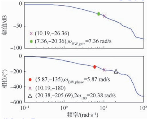
图 8 俯仰通道频响 Fig. 8 Frequency response of pitch channel
