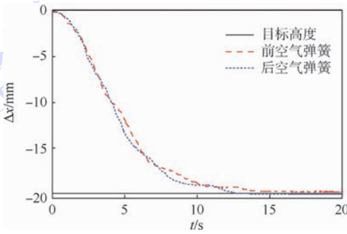
图 8 中位到低位车身高度调节试验结果 Fig. 8 Test results of vehicle height adjustment from normal mode to low mode
