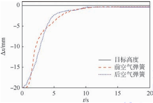
图 6 低位到中位车身高度调节试验结果 Fig. 6 Test results of vehicle height adjustment from low mode to normal mode
