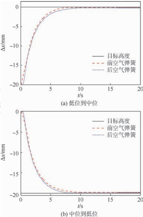
Δx—空气弹簧高度变化;t—时间. 图 4 低位到中位和中位到低位车身高度调节仿真结果 Fig.4 Simulation results of vehicle height adjustment from low mode to normal mode and from normal mode to low mode
