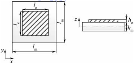
x, y, z —板的坐标轴; l_e, l_m —压电片长和板长; h_e, h_m —压电片高和板高.
