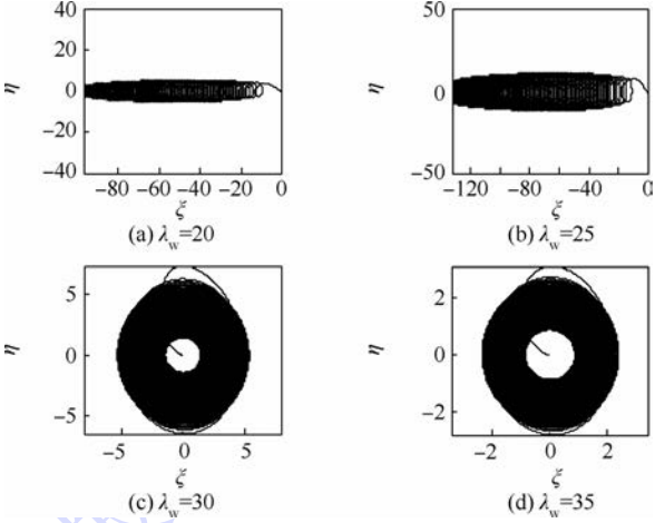
图 25 非对称 ( \kappa = 0.03 ) 厚盘转子定功率过高阶临界转速时盘偏角矢尖轨迹 Fig. 25 Trajectories of declination angle vector tip of disk of asymmetric thick-disk rotor ( \kappa = 0.03 ) crossing higher order critical speed with constant power
