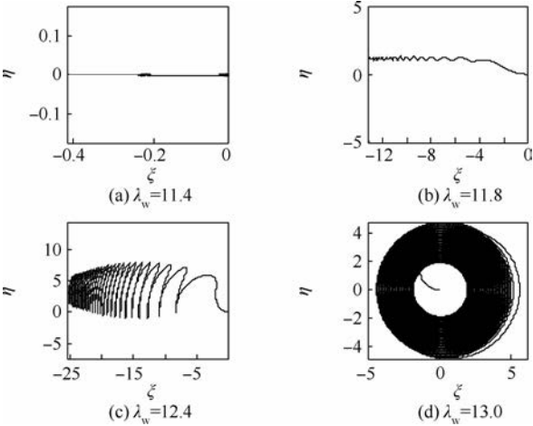
图 23 对称厚盘转子定功率过高阶临界转速时盘偏角矢尖轨迹 Fig. 23 Trajectories of declination angle vector tip of disk of symmetric thick-disk rotor crossing higher order critical speed with constant power
