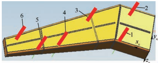
图 17 各个油箱两根传感器的优化布局结果三维图 Fig. 17 Three-dimensional diagram of optimal layout results of each fuel tank with two sensors
