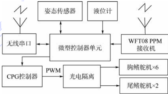
图 3 硬件架构 Fig. 3 Hardware configuration
