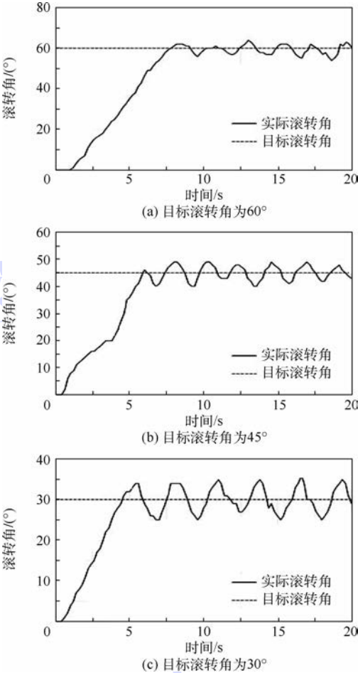
图 11 滚转角随时间变化曲线 Fig. 11 Curve of roll angle changing with time
