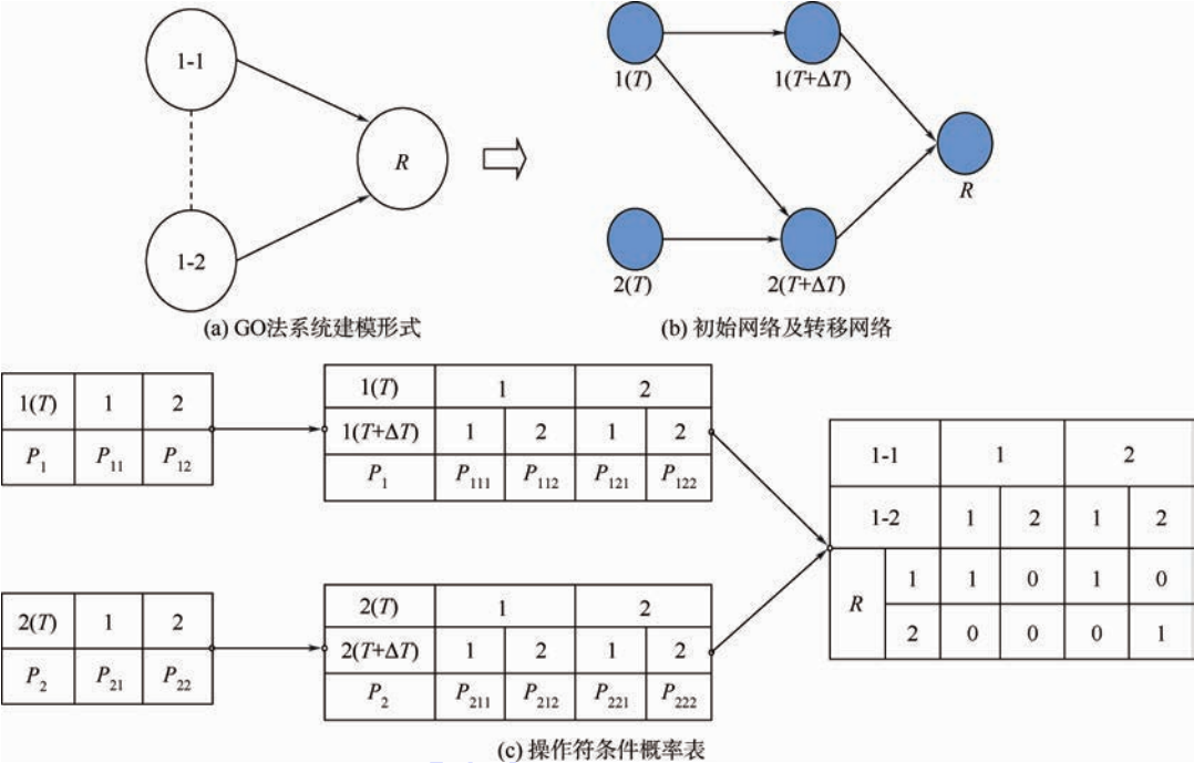
图 9 操作符之间的备用相关 Fig. 9 Standby dependence between operators
