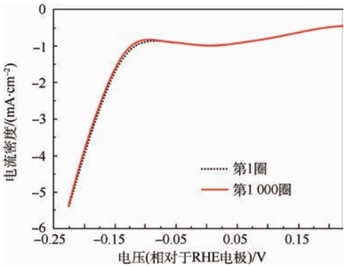
图 6 MoS 2 /Graphene 电催化剂的稳定性测试 Fig. 6 Durability test for MoS 2 /Graphene electrocatalyst
