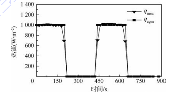
图 6 数值试验 2 的吸收外热流反演值与真实值比较 Fig. 6 Compare between inversion absorbed external heat flux and real value of numerical experiment 2
