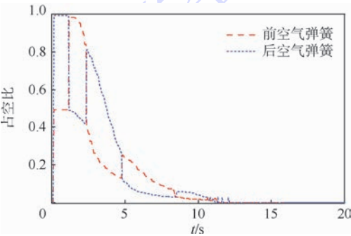
图 7 低位到中位车身高度调节占空比信号试验结果 Fig. 7 Test results of the duty cycle signal during vehicle height adjustment from low mode to normal mode
