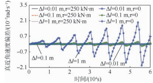
图 14 系绳长度偏差对 CCPTS 真近角速度的影响 Fig. 14 Influence of tether length deviation on true anomaly angular velocity of CCPTS
