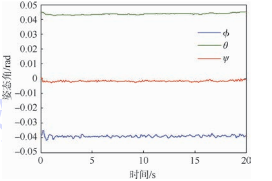
图 17 风扰下的姿态保持 Fig. 17 Attitude hold with wind disturbance
