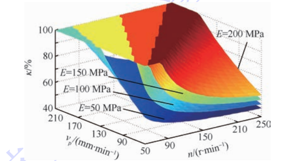
图 16 取心率与模拟月壤弹性模量关系 Fig. 16 Relation between coring rate and elastic modulus of lunar soil simulant
