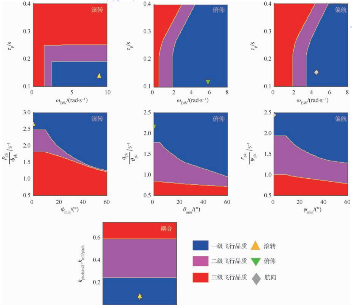
图 18 姿态控制器飞行品质评估结果汇总 Fig. 18 Summary of flight quality evaluation results for attitude controller
