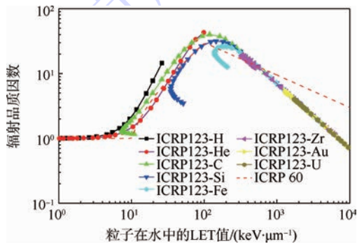
图3 ICRP 123 与 ICRP 60 出版物的辐射品质因数 Fig.3 Radiation quality factor from ICRP 60 and ICRP 123 publications
