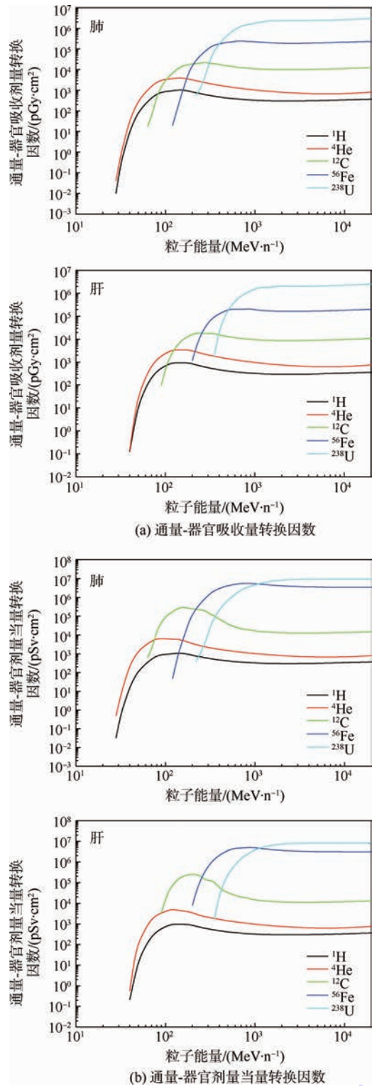
图 5 受 1 H、 4 He、 12 C、 56 Fe 和 238 U 粒子照射时通量-器官吸收剂量转换因数和通量-器官剂量当量转换因数 Fig. 5 Fluence to organ absorbed dose conversion coefficients and organ dose equivalent conversion coefficients for exposure by 1 H, 4 He, 12 C, 56 Fe and 238 U
