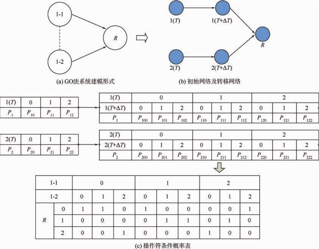
图 10 操作符之间的维修相关 Fig. 10 Repair dependence between operators
