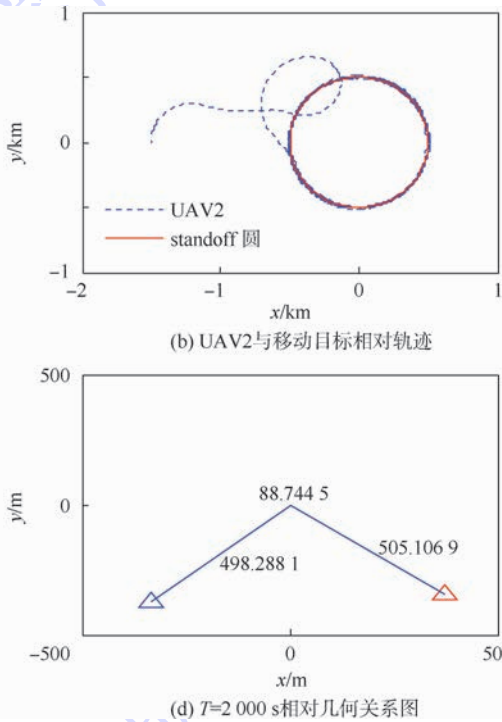
图 4 UAV 与目标的瞬时相对轨迹和几何关系 Fig.4 Relative trajectories between UAV and target and their instantaneous geometric relationships
