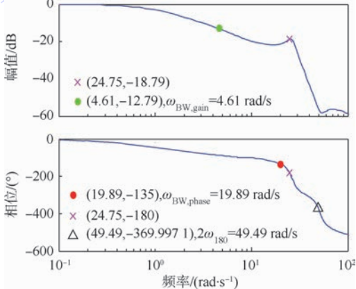
图 9 偏航通道频响 Fig. 9 Frequency response of yaw channel
