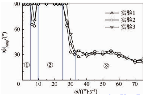
图 4 摇摆运动振幅随攻角拉起速度的变化曲线 Fig. 4 Curves of amplitude of free-to-roll motion changing with pitch rate
