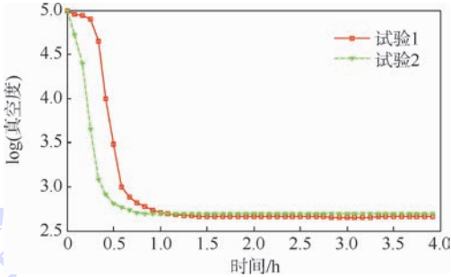
图 7 温度对真空度的影响 Fig. 7 Vacuum degree influenced by temperature
