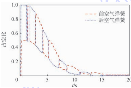
图 9 中位到低位车身高度调节占空比信号试验结果 Fig. 9 Test results of the duty cycle signal during vehicle height adjustment from normal mode to low mode
