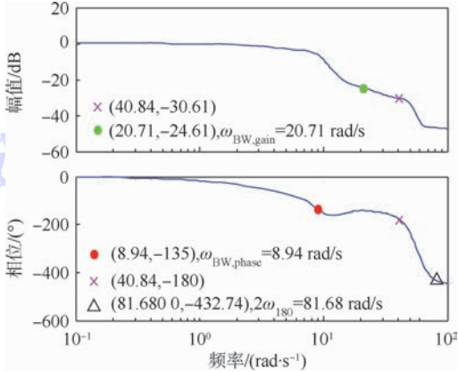
图 7 滚转通道频响 Fig. 7 Frequency response of roll channel
