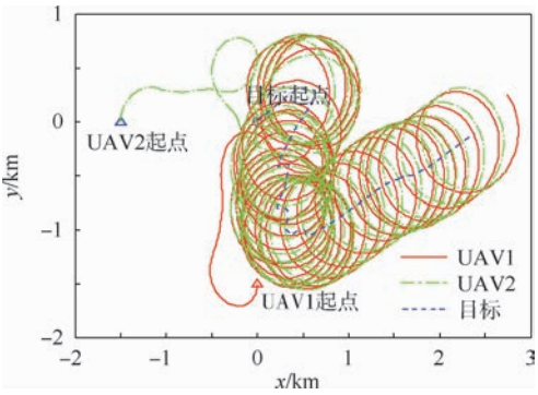
图 2 两架 UAV 与随机运动目标的绝对航迹 Fig.2 Absolute trajectories of two UAVs and random moving target
