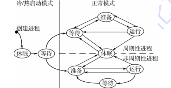
图 8 进程状态转移 Fig.8 Process states transform
