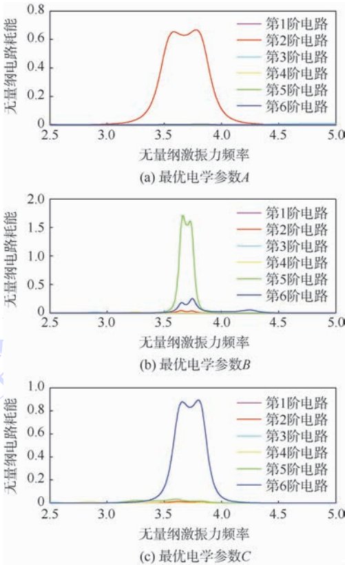
图 10 各阶电路系统耗能对比 Fig. 10 Comparison of energy dissipation in electrical system among different orders
