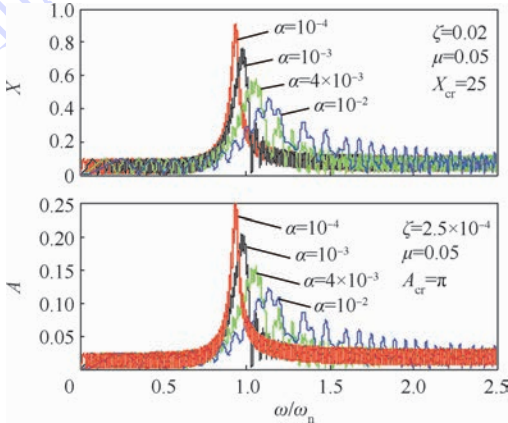
图 7 计重力厚盘转子过低阶临界转速的瞬态振动曲线 Fig.7 Transient vibration curves of thick-disk rotor crossing lower order critical speed with gravity taken into account
