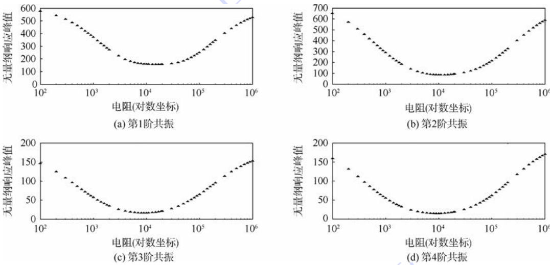
图 6 电阻对共振峰值的影响 (R-PEM) Fig. 6 Influence of resistance on resonance peak value (R-PEM)
