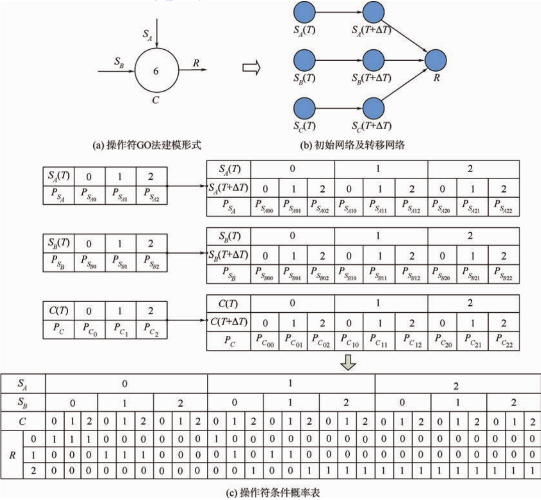
图 7 第 6 类操作符及对应动态贝叶斯网络 Fig.7 Type 6 operator and its dynamic Bayesian network
