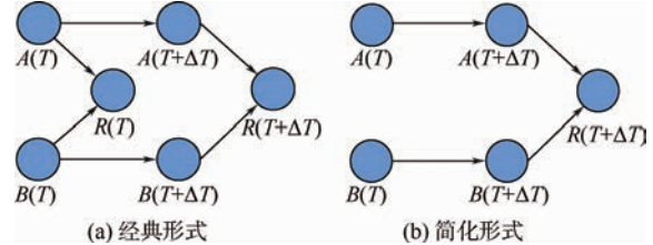
图 2 “与”逻辑对应的动态贝叶斯网络 Fig. 2 Dynamic Bayesian network of logic “AND”
