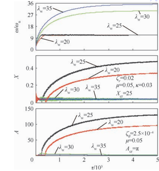
图 24 非对称 ( \kappa = 0.03 ) 厚盘转子定功率过高阶临界转速时随时间变化的瞬态振动曲线 Fig. 24 Transient vibration curves over time of asymmetric thick-disk rotor ( \kappa = 0.03 ) crossing higher order critical speed with constant power
