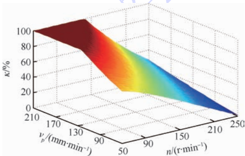
图 18 无外伸管钻头取心率与钻进规程参数关系 Fig. 18 Relation between coring rate and drilling parameters for non-extended tube drill bit
