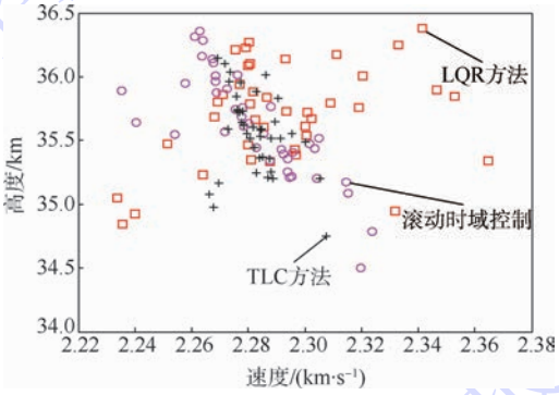
图 4 速度-高度剖面打靶结果 Fig. 4 Shooting results in velocity-altitude profile
