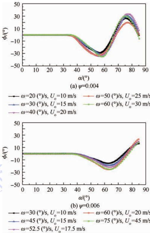
图 6 不同拉起减缩频率下的摇摆运动 Fig. 6 Free-to-roll motions for different reduced frequencies
