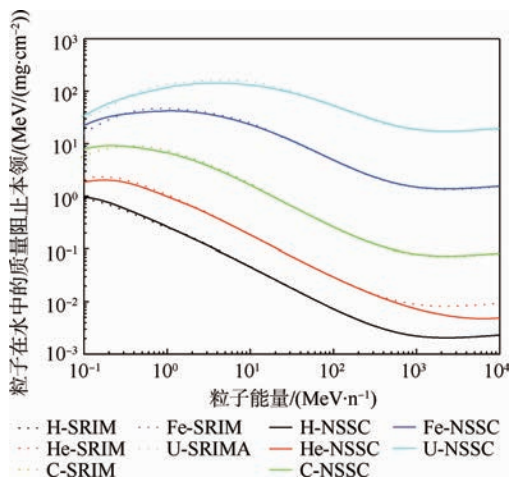
图2 不同粒子在水中的质量阻止本领 Fig.2 Stopping powers of various particles in water
