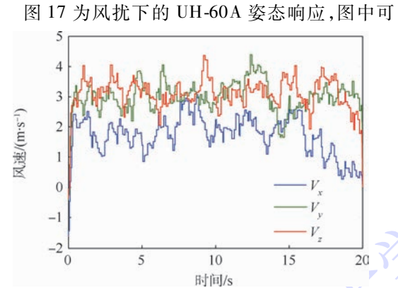
图 16 地面坐标系下的风扰动 Fig. 16 Wind disturbance in ground coordinate system
