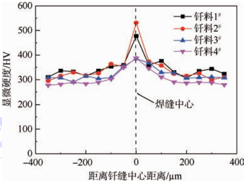
图 5 不同钎料钎焊接头的显微硬度分布 Fig. 5 Distribution of microhardness of brazed joints with different filler metals
