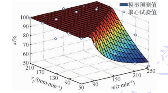
图 14 取心率计算值与试验值对比 Fig. 14 Comparison between calculation and test results of coring rate
