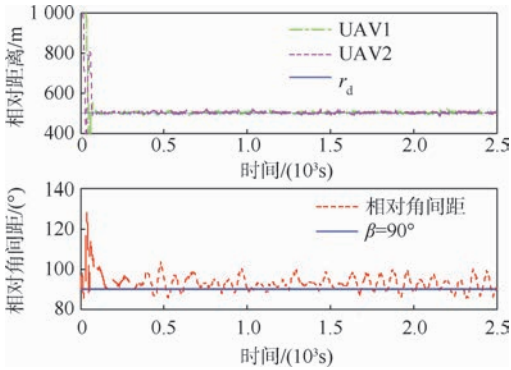
图 3 UAV 与随机运动目标相对距离和相对角间距 Fig.3 Relative distances and angle spacing between UAV and random moving target
