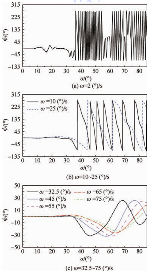
图 5 不同拉起速度下摇摆运动随攻角的变化曲线 Fig. 5 Curves of free-to-roll motion changing with angle of attack for different pitch rates
