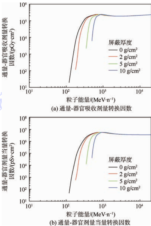
图 6 不同屏蔽厚度下 56 Fe 粒子照射时的通量-器官吸收剂量转换因数和通量-器官剂量当量转换因数 Fig. 6 Fluence to organ absorbed dose conversion coefficients and organ dose equivalent conversion coefficients for exposure by 56 Fe with various shielding thicknesses
