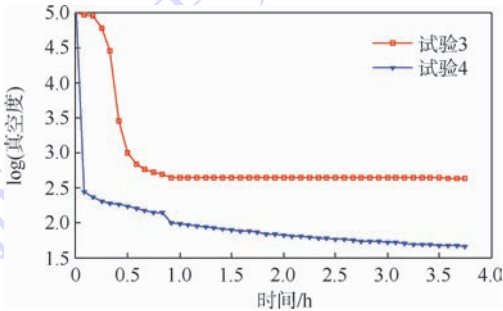
图 8 抽速对真空度的影响 Fig. 8 Vacuum degree influenced by pumping velocity
