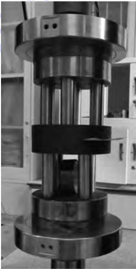
图 4 紧固件拉拔试验夹具 Fig.4 Fixture of fastener tensile test
