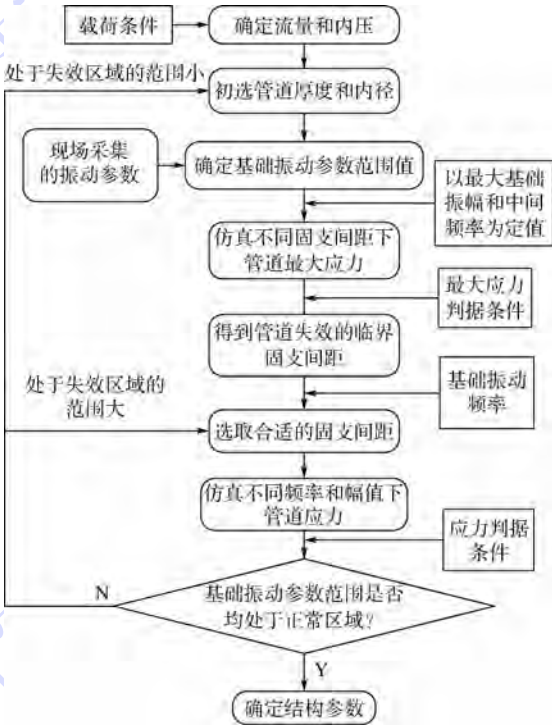
图 9 强振动环境下抗振结构设计流程图 Fig. 9 Design flow chart of anti-vibration structure in strong vibration environment
