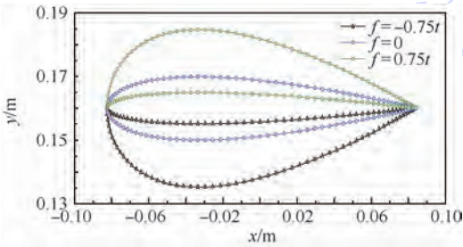
图 6 拱度为 -0.75t 、0 和 0.75t 时导管翼形剖面示意图 Fig. 6 Schematic diagram of duct's airfoil sections as f = -0.75t , f = 0 , and f = 0.75t
