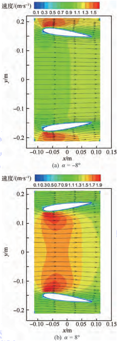
图 16 \alpha = -8^\circ 和 \alpha = 8^\circ 时导管 O-xy 截面 上流线和轴向速度分布 Fig. 16 Flow lines and axial velocity distribution on O-xy section as \alpha = -8^\circ and \alpha = 8^\circ
