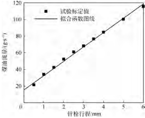
图3 可调文氏管流量 Fig.3 Mass flow rate of adjustable venturi
