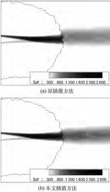
图 9 2 种插值方法的尾涡无量纲黏性分布对比 Fig. 9 Rear eddy nondimensional viscosity contour distribution comparison of two interpolation methods
