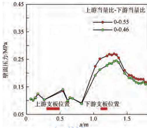
图 7 Case 2 不同下游当量比壁面压力分布 Fig. 7 Wall pressure distribution of Case 2 with different downstream equivalence ratios
