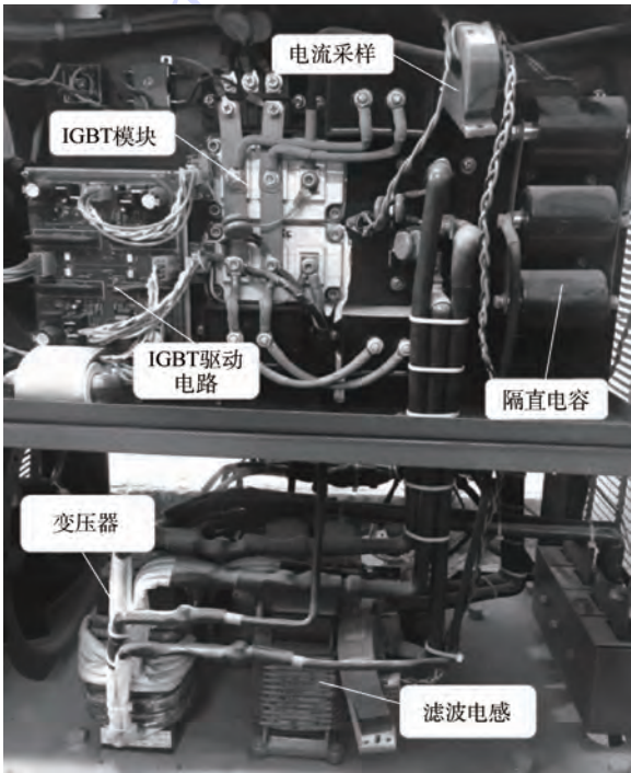
图 4 DC-DC 全桥变换器实物 Fig. 4 Real products of DC-DC full-bridge converter
