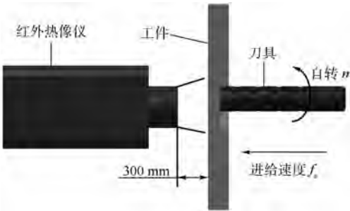
图 2 切削温度测温方法示意图 Fig. 2 Schematic diagram of cutting temperature measurement method
