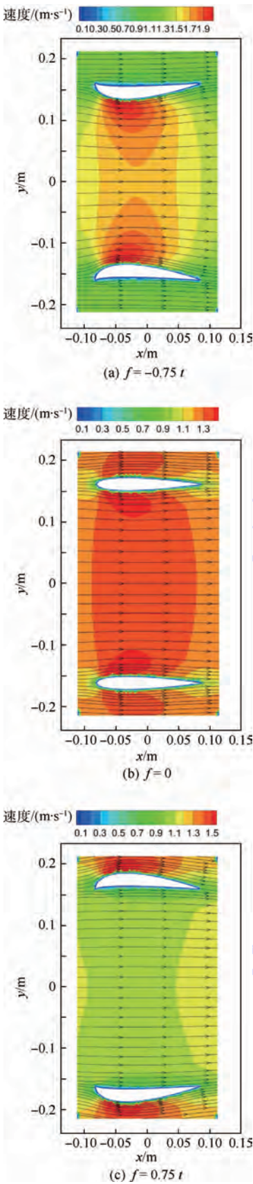
图 8 f = -0.75t 、 f = 0 和 f = 0.75t 时导管 O - xy 截面上流线和轴向速度分布 Fig. 8 Flow lines and axial velocity distribution on O - xy section as f = -0.75t , f = 0 , and f = 0.75t
