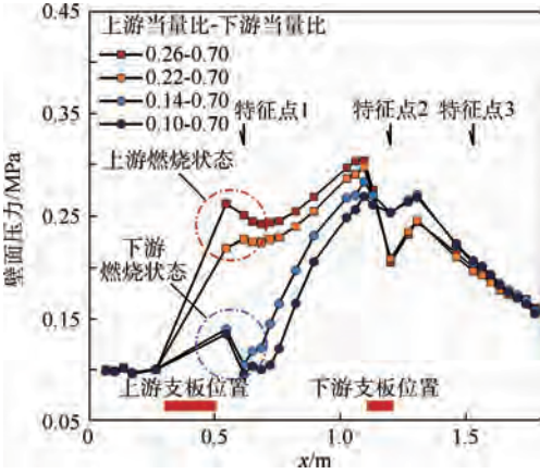
图4 Case 1 不同上游当量比壁面压力分布 Fig. 4 Wall pressure distribution of Case 1 with different upstream equivalence ratios
