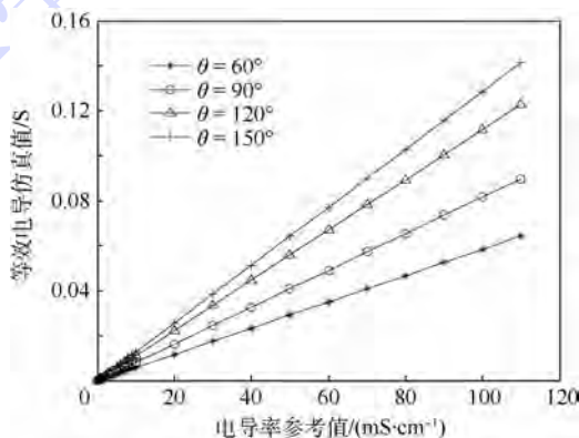
图 6 电极片张角改变时两电极间等效电导仿真值 Fig.6 Simulation equivalent conductivity value between two electrodes when angle of electrode changes
