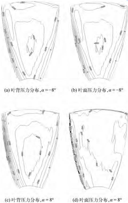
图 20 \alpha = -8^{\circ} 、 \alpha = 8^{\circ} 时桨叶的叶背、叶面压力分布 Fig. 20 Pressure distribution on propeller's back and face as \alpha = -8^{\circ} and \alpha = 8^{\circ}
