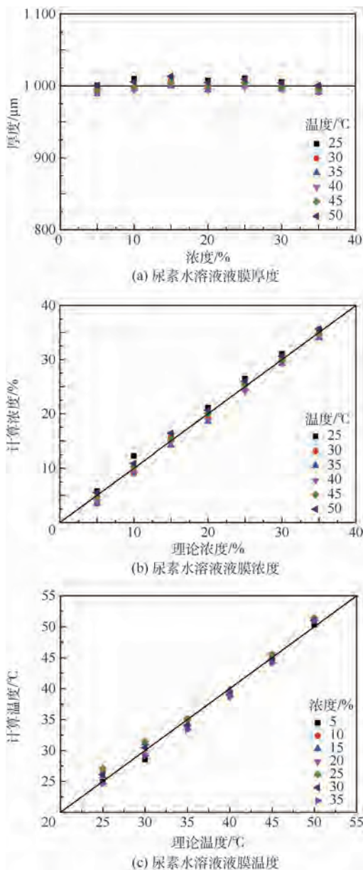
图 3 尿素水溶液液膜厚度、浓度及温度反演结果 Fig. 3 Calculated results of film thickness, mass fraction and temperature for urea-water-solution
