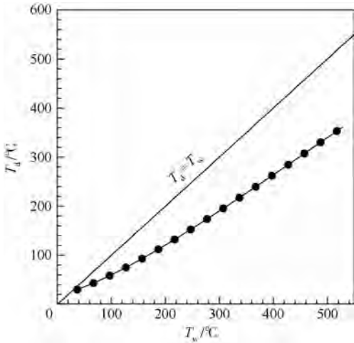
图 7 红外 CCD 相机探测温度随表面真实温度的变化曲线 Fig. 7 Variation curve of detected temperature measured by infrared CCD camera with surface real temperature
