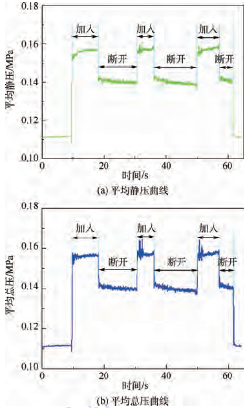
图 8 补燃室的平均静压和平均总压曲线 Fig.8 Average static and total pressure curves of afterburning chamber
