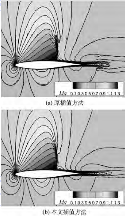
图 7 2 种插值方法的马赫数分布比较 Fig. 7 Mach number contour distribution comparison of two interpolation methods
