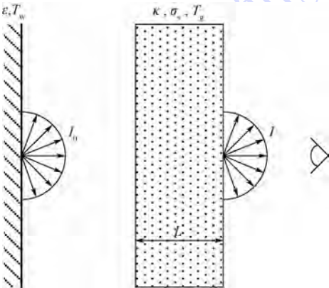
图 5 一维大平板红外测温模型示意图 Fig. 5 Schematic of infrared temperature measurement for 1D plane-parallel slab model
