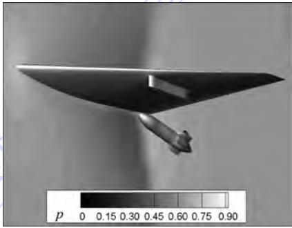
图 12 0.3 s 时刻对称面和物面压力分布 Fig. 12 Surface and symmetry pressure contour at 0.3 s
