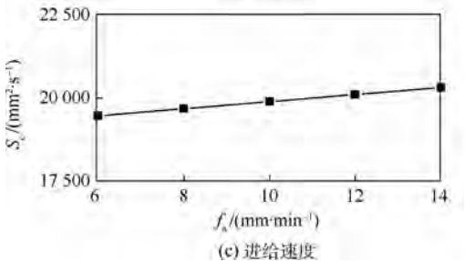
图7 不同自转转速、公转转速及进给速度下未变形切屑面积 Fig.7 Undeformed chip area under different spindle speeds, orbital speeds and feed speeds
