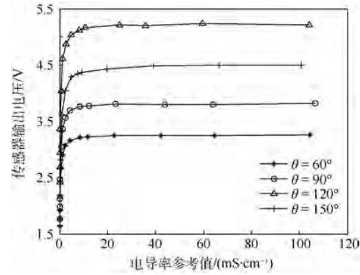
图7 不同电极张角时传感器的输出特性 Fig.7 Output characteristics of sensors with different electrode angles
