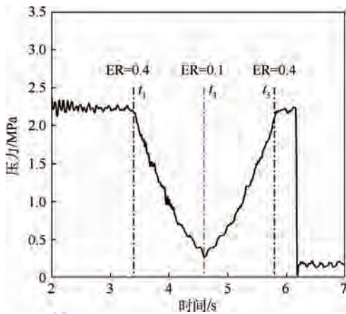
图 12 Case 6 文氏管后压力随时间的变化 Fig. 12 Time history of pressure after venturi of Case 6
