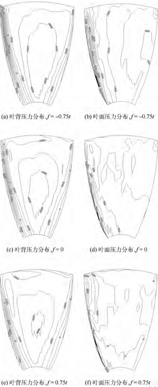
图 12 f = -0.75t 、 f = 0 和 f = 0.75t 时 桨叶的叶背、叶面压力分布 Fig. 12 Pressure distribution on propeller's back and face as f = -0.75t , f = 0 and f = 0.75t
