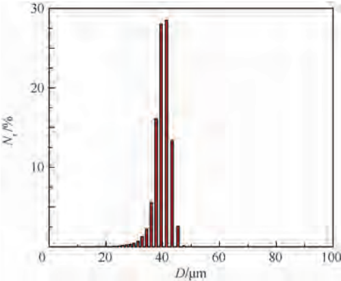
图 6 39.2 μm 乳胶球的粒径概率分布 Fig. 6 Particle size probability distribution of 39.2 μm latex spheres
