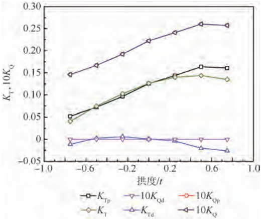
图 11 导管翼形剖面拱度对螺旋桨水动力性能的影响 Fig. 11 Influences of cambers of duct's airfoil section on propeller's hydrodynamic performance
