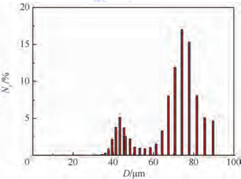
图 9 混合乳胶球的粒径概率分布 Fig. 9 Particle size probability distribution of mixture latex spheres
