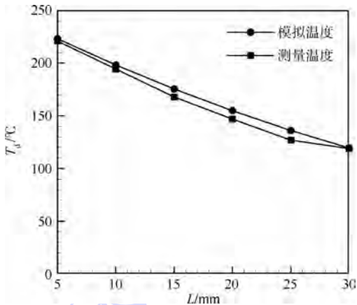
图 8 不同振动筛宽度下测量与模拟的表面温度比较 Fig. 8 Comparison between measured and calculated temperatures of surface at different widths of vibrating screen
