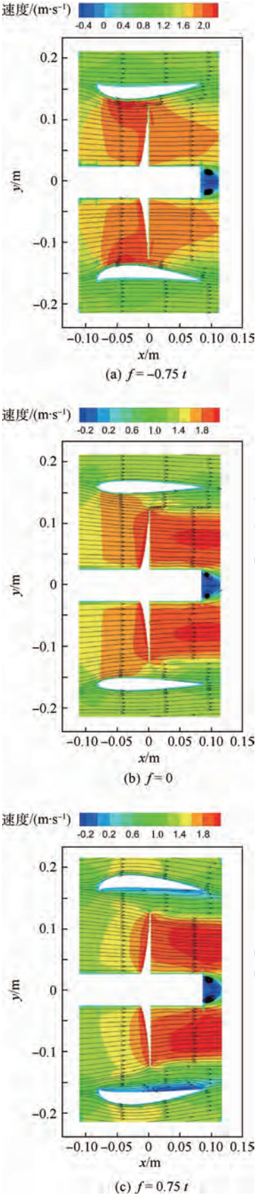
图 10 f = -0.75 t 、 f = 0 和 f = 0.75 t 时导管桨 O-xy 截面上流线和轴向速度分布 Fig. 10 Flow lines and axial velocity distribution on O-xy section with propeller as f = -0.75 t , f = 0 , and f = 0.75 t
