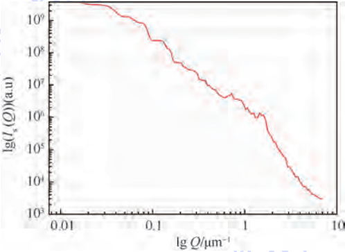
图 8 混合乳胶球的散射光强分布 Fig. 8 Scattered intensity distribution of mixture latex spheres
