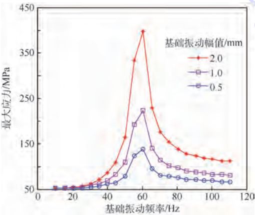
图 7 最大应力随基础振动频率变化规律 Fig. 7 Change rules of maximum stress with foundation vibration frequency
