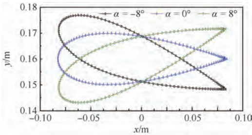
图 15 \alpha = -8^\circ 、 \alpha = 0^\circ 和 \alpha = 8^\circ 时导管翼形剖面示意图 Fig. 15 Schematic diagram of duct's airfoil sections as \alpha = -8^\circ , \alpha = 0^\circ , and \alpha = 8^\circ
