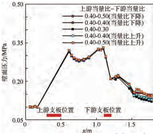
图 11 Case 5 不同下游当量比壁面压力分布 Fig. 11 Wall pressure distribution of Case 5 with different downstream equivalence ratios
