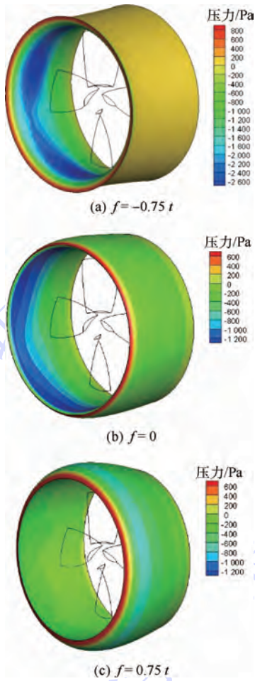
图 13 f = -0.75t 、 f = 0 和 f = 0.75t 时导管压力分布 Fig. 13 Pressure distribution on duct as f = -0.75t , f = 0 , and f = 0.75t
