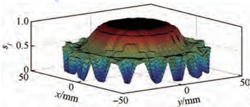
图9 管道内超声灵敏度分布 Fig.9 Ultrasonic sensitivity distribution inside pipeline
