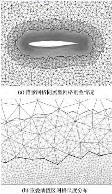
图 6 RAE2822 翼型重叠网格 Fig. 6 Overset grid of RAE2822 wing figure
