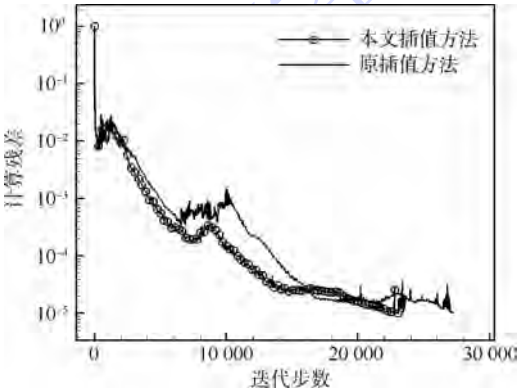
图 10 2 种插值方法的残差收敛情况对比 Fig. 10 Comparison of residual error convergence history of two interpolation methods
