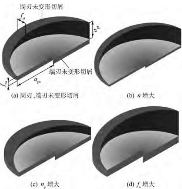
图6 未变形切屑 Fig.6 Undeformed chip
