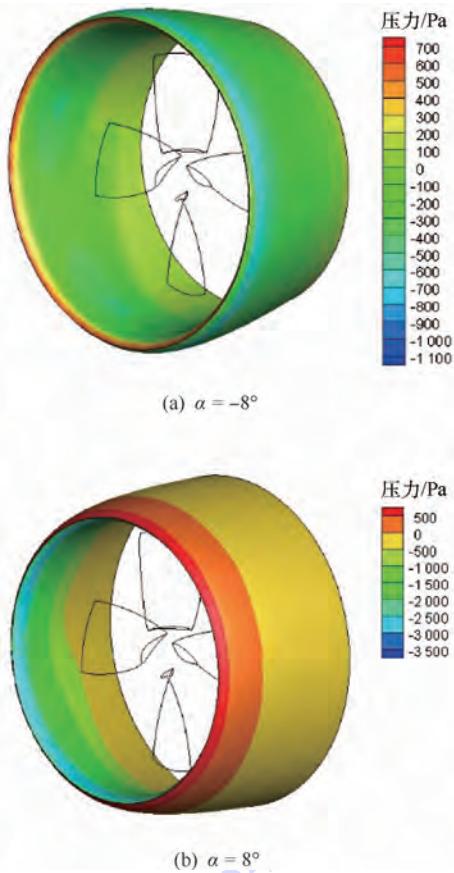
图 21 \alpha = -8^{\circ} 和 \alpha = 8^{\circ} 时导管压力分布 Fig. 21 Pressure distribution on duct as \alpha = -8^{\circ} and \alpha = 8^{\circ}
