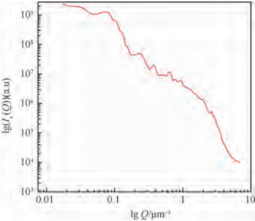
图 5 39.2 μm 乳胶球的散射光强分布 Fig. 5 Scattered intensity distribution of 39.2 μm latex spheres
