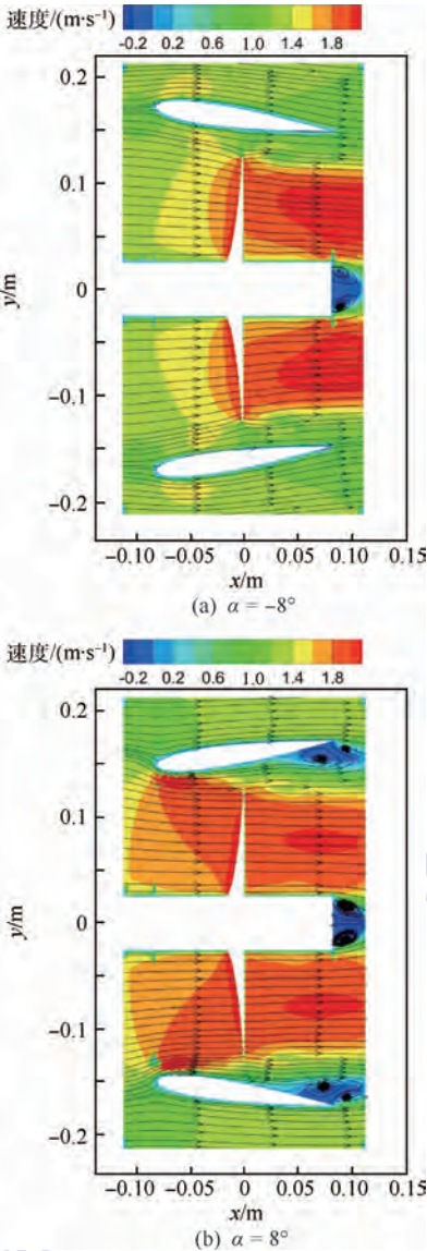
图 18 \alpha = -8^\circ 和 \alpha = 8^\circ 时导管 O - xy 截面上流线和轴向速度分布 Fig. 18 Flow lines and axial velocity distribution on O - xy section as \alpha = -8^\circ and \alpha = 8^\circ
