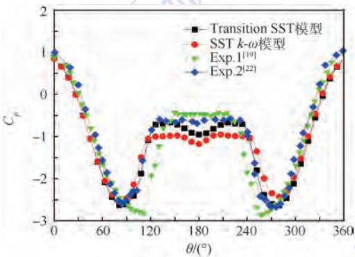
图 7 在临界区圆柱表面时均压力系数 C_p 分布曲线 Fig. 7 Distribution curves of time-averaged pressure coefficient C_p on cylindrical surface in critical region
