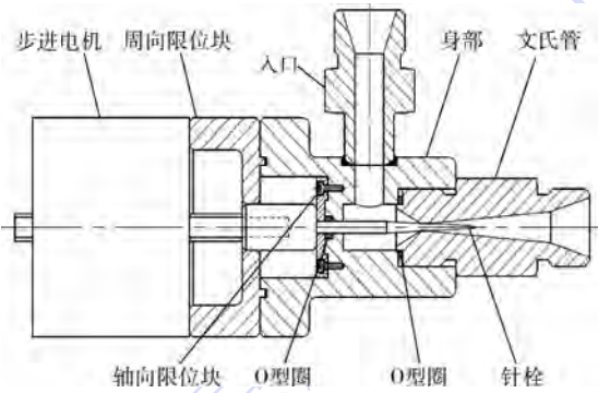
图2 可调文氏管结构 Fig.2 Structure of adjustable venturi
