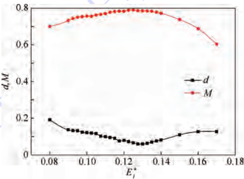
图10 电极相对宽度对超声场平均灵敏度与标准差的影响 Fig.10 Influence of relative electrode width on average sensitivity and standard deviation of ultrasonic field
