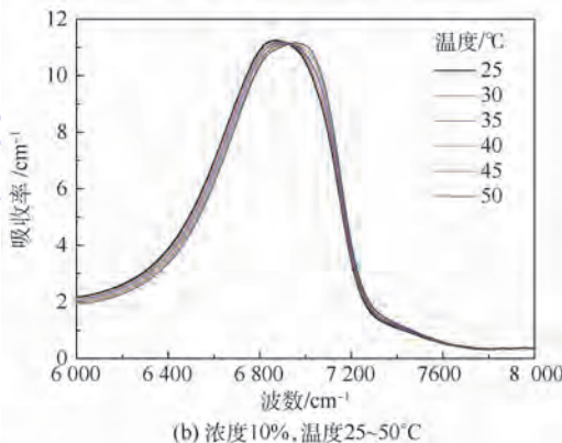
图1 温度 30^\circ\text{C} , 不同浓度( 5\% \sim 35\% )以及浓度 10\% 不同温度( 25 \sim 50^\circ\text{C} )的尿素水溶液吸收光谱 Fig.1 Absorption spectra of urea-water-solution with different mass fraction ( 5\% \sim 35\% ) at 30^\circ\text{C} and with mass fraction of 10\% at different temperature ( 25 \sim 50^\circ\text{C} )
