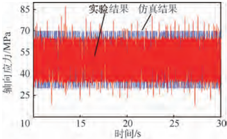
图6 应力仿真曲线及与实验结果局部对比图 Fig.6 Local contrast chart of stress simulation curves and experimental results
