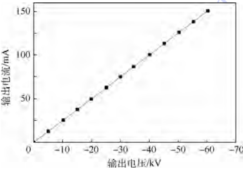
图 11 负载为 400 kΩ 时电源输出特性 Fig. 11 Output characteristics of high-voltage power supply with load 400 kΩ
