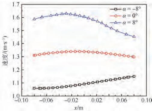
图 17 \alpha = -8^\circ 、 \alpha = 0^\circ 和 \alpha = 8^\circ 时导管内 沿中轴线的轴向速度分布 Fig. 17 Axial velocity distribution along x -axis as \alpha = -8^\circ , \alpha = 0^\circ , and \alpha = 8^\circ
