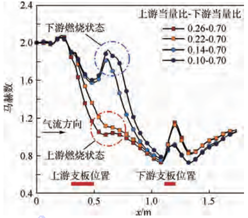
图5 Case 1 不同上游当量比马赫数分布 Fig. 5 Mach number distribution of Case 1 with different upstream equivalence ratios
