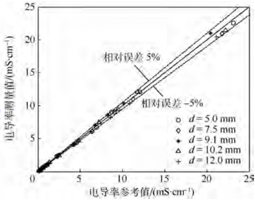
图8 电导率测量实验结果 Fig.8 Experimental results of conductivity measurement
