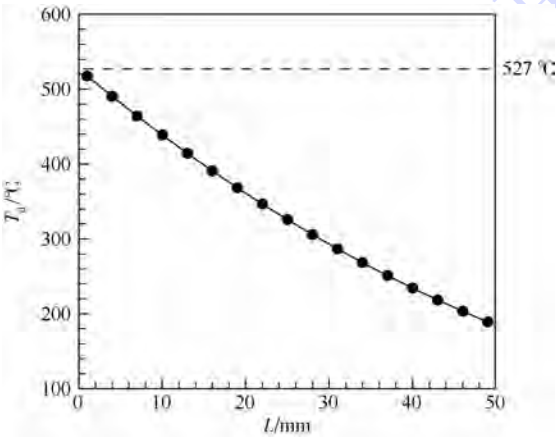
图 6 红外 CCD 相机探测温度随振动筛宽度的变化曲线 Fig. 6 Variation curve of detected temperature measured by infrared CCD camera with width of vibrating screen
