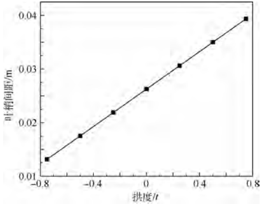
图 7 叶梢间距随导管拱度的变化 Fig. 7 Variation of tip clearance with cambers of duct
