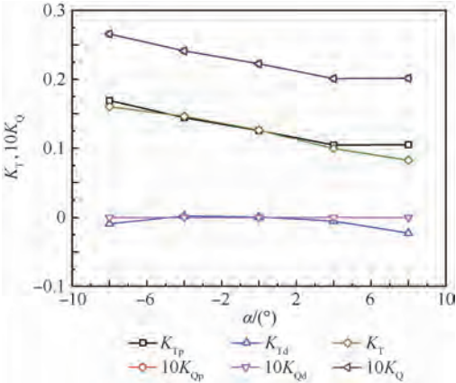
图 19 导管翼型剖面攻角对螺旋桨水动力性能的影响 Fig. 19 Influences of attack angles of duct's airfoil section on propeller's hydrodynamic performance
