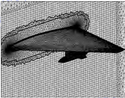
图 11 三维机翼挂架重叠网格 Fig. 11 3D overset grid of wing/pylon/store
